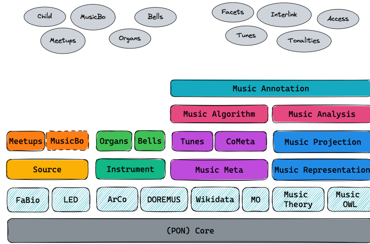
Fig. 3. Overview of the main modules in the Polifonia Ontology Network, with Polifonia’s pilots as early adopters (grey circles). Foundational models ( Source , Instrument , Music Meta , Music Representation ) provide the backbone of PON, built on top of the Core module while leveraging the main ontologies reused directly or indirectly.
